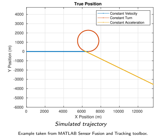
Example taken from MATLAB Sensor Fusion and Tracking toolbox.
